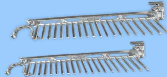
Hose Rack Size : 1.5" & 2.5" Material : Brass & Chrome Pressure Test : 10 bar & 16 bar
